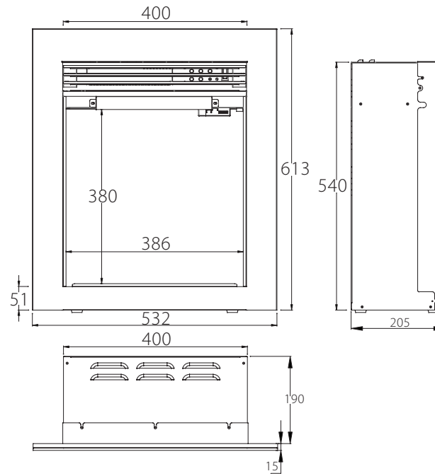
Iconic 400 Slim & Trance 400
