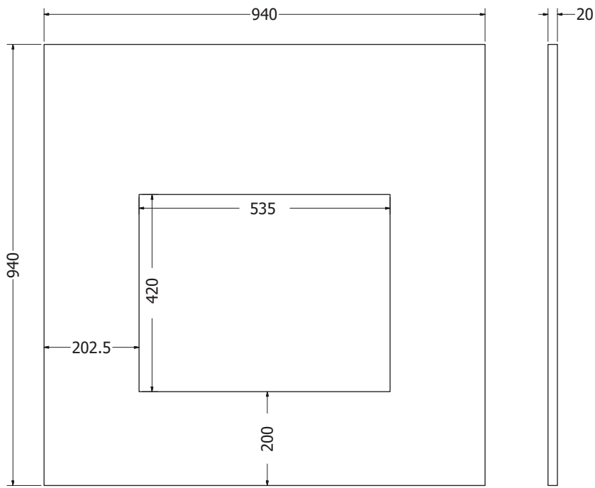
Iconic 530 Black Granite Back Panel
