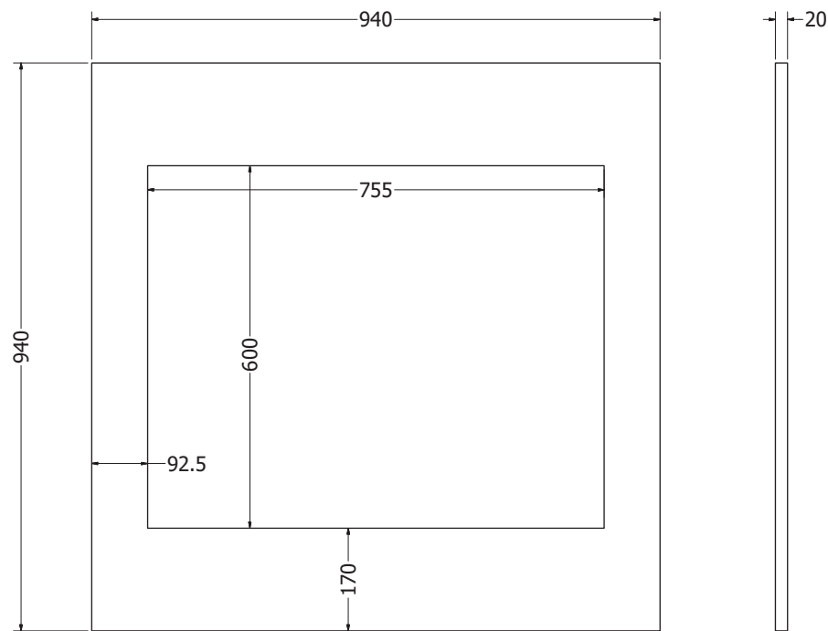
Iconic 750 Black Granite Back Panel
