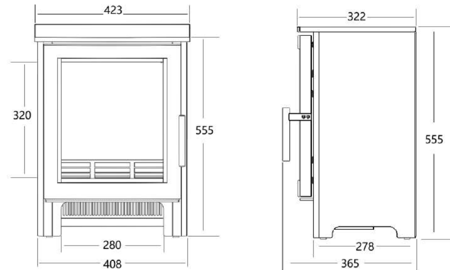
Iconic 500 Electric Stove
